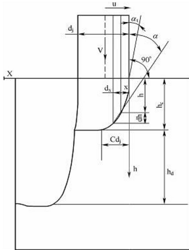
Figure 4. Details of the kerf geometry on a workpiece
