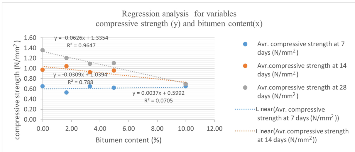
Figure 4. Scatter plot showing the relationship between compressive strength and bitumen content for block sets.
