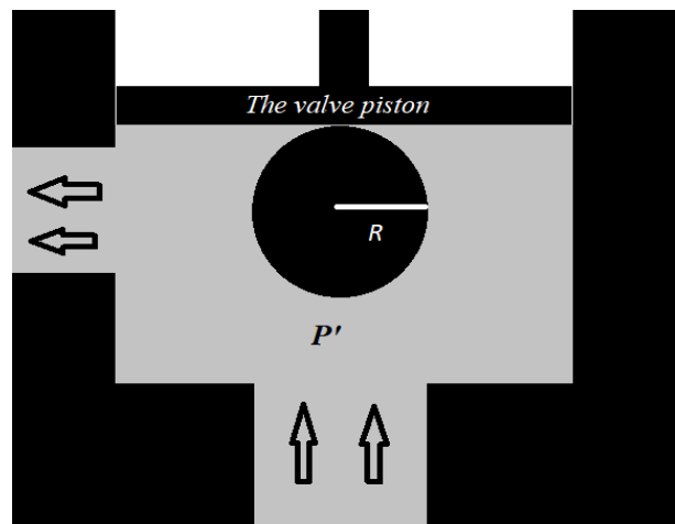
Figure 6. The steel ball and the piston of the fuel overflow valve when it is activated
