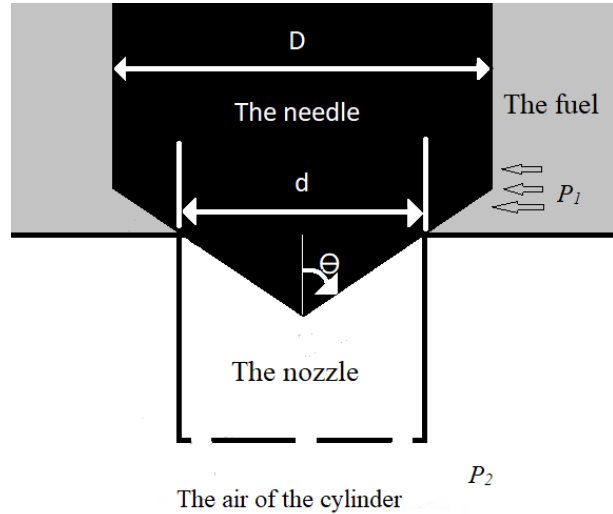
Figure 1. The injector needle and nozzle before the injection
