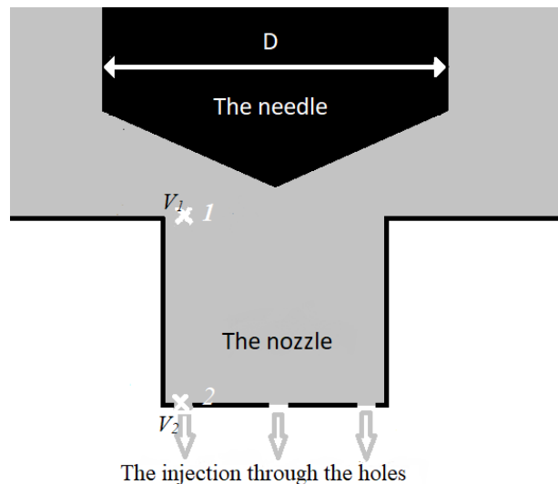
Figure 2. The injector needle and nozzle during the injection
