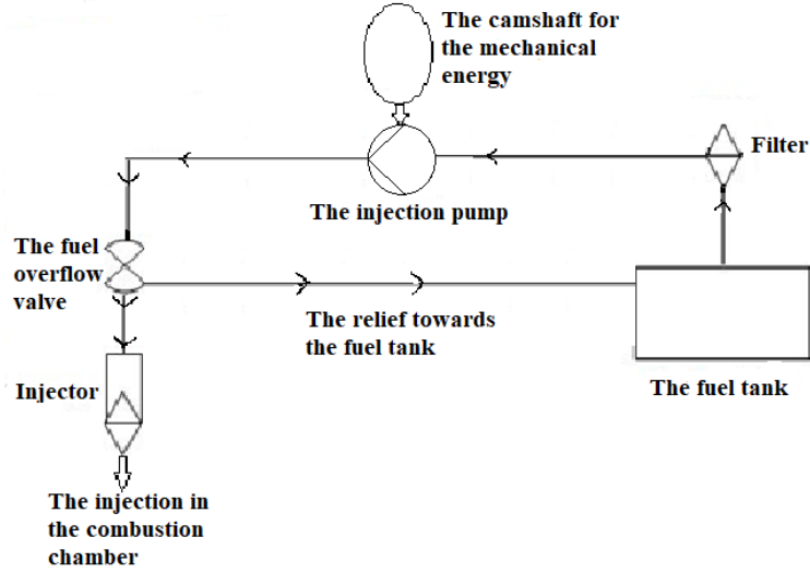
Figure 7. A schematic diagram of the fuel injection system
