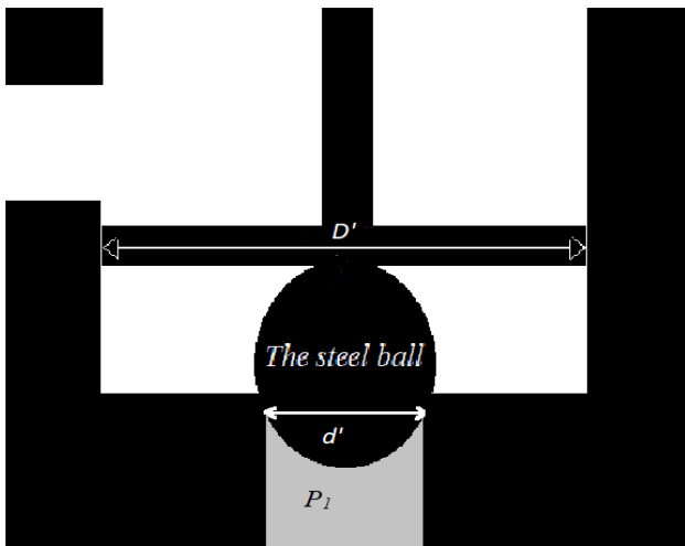
Figure 4. The steel ball and the piston of the fuel overflow valve before it is activated
