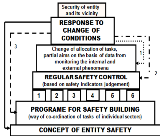
Figure 6. Safety management system of technological facility [25]
