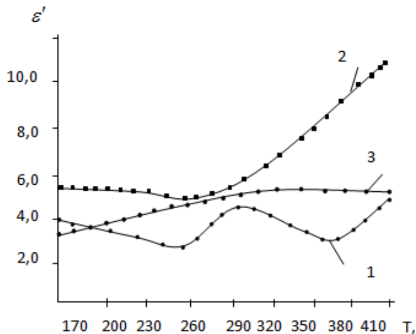
Figure 1. The dependence on T for PMMA at frequency of 50kHz. 1 -- initial, 2 - 30 hours, 3 - 2 months after irradiation. J_{imp} = 5 \text{ kW} / \text{cm}^2 .
