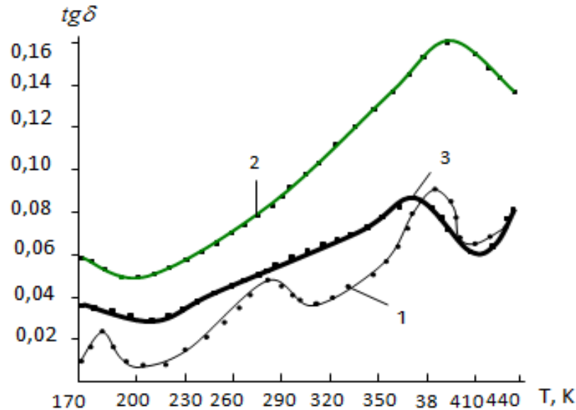
Figure 2. The dependence of the tangent dielectric loss angle of temperature for PMMA at frequency of 50kHz. 1 - initial, 2 - 30 hours, 3 - 2 months after irradiation. I_{\text{imp}} \text{ и ч. } I=5\text{kW} / \text{cm}^2
