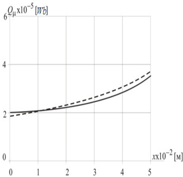
Figure 4. The curves of change of the magnetic flux along the magnetic circuit: solid line - estimated; the dotted line – pilot
