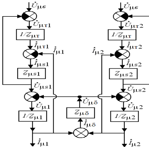
Figure 2. PSD of the magnetic circuit of electromagnetic transducers
