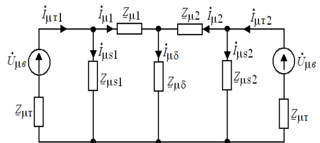
Figure 1. The equivalent circuit of the magnetic circuit of the electromagnetic transducers of three-phases current
