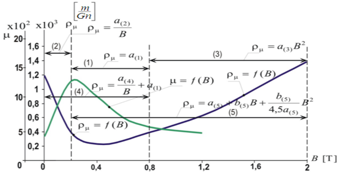
Figure 3. Curves and specific magnetic resistance of the magnetic permeability of steel from induction
