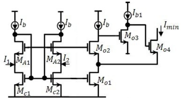
Figure 4. The proposed Minimum current selector
