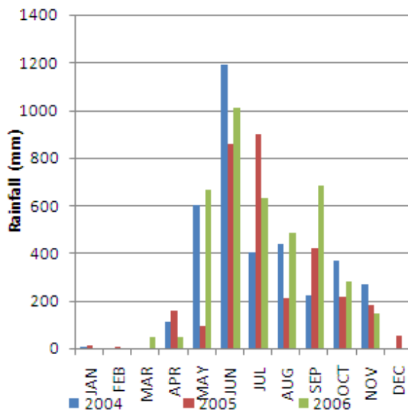
Figure 1. Monthly average rainfall data of Kerala for three consecutive years [9].
