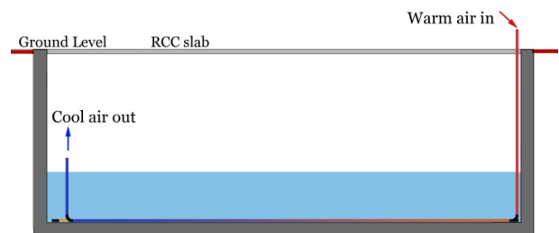
Figure 6. Section of the tank and layout of the pipes
