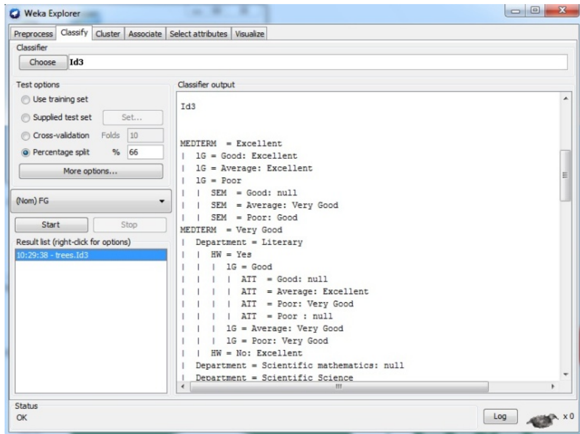
Figure 4. Midterm as root node
