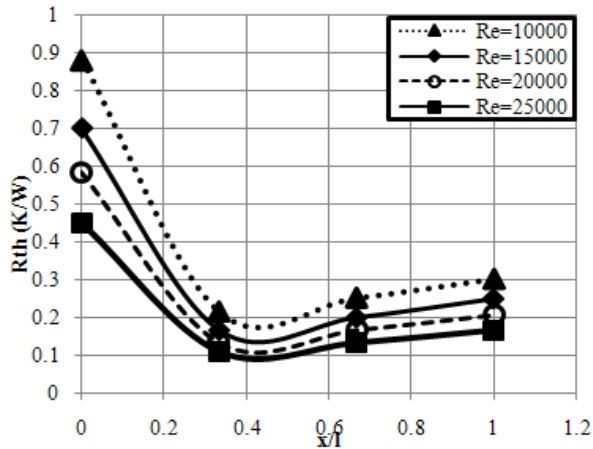
Figure 10. Distribution of thermal resistance with shield position at different Reynolds numbers
