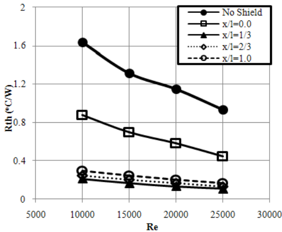
Figure 7. Thermal resistance versus Reynolds numbers at different shield positions
