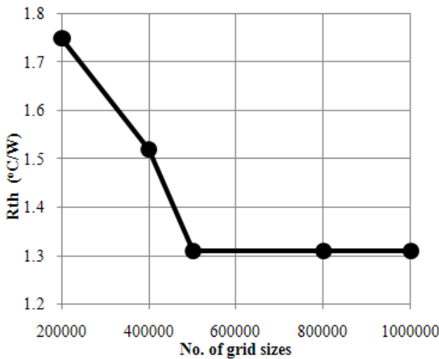
Figure 3. Thermal resistance at different grid sizes
