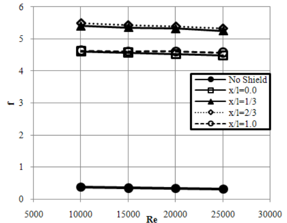
Figure 9. Variation of friction factors with Reynolds numbers at different shield position
