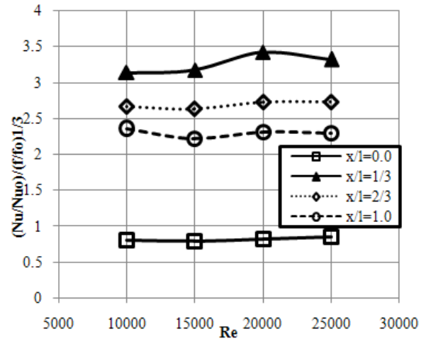
Figure 11. Performance evaluations of fin array with different shield positions, under identical pumping power criterion
