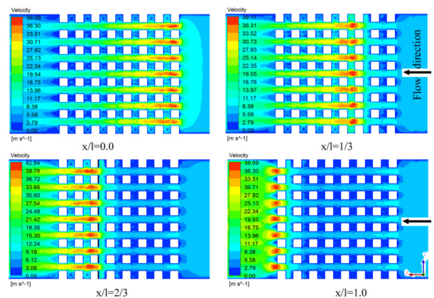
Figure 5. Velocity distribution at y = 0.01 m at various shield positions for Re = 25000
