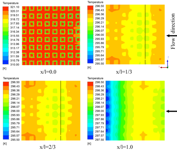
Figure 6. Temperature distribution over heat sink base at various shield position for Re = 25000
