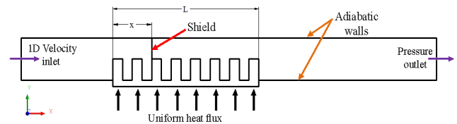
Figure 2. Computational domain and boundary conditions
