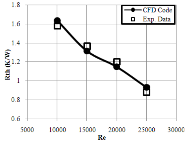
Figure 4. Comparison between present experimental measurements and numerical code
