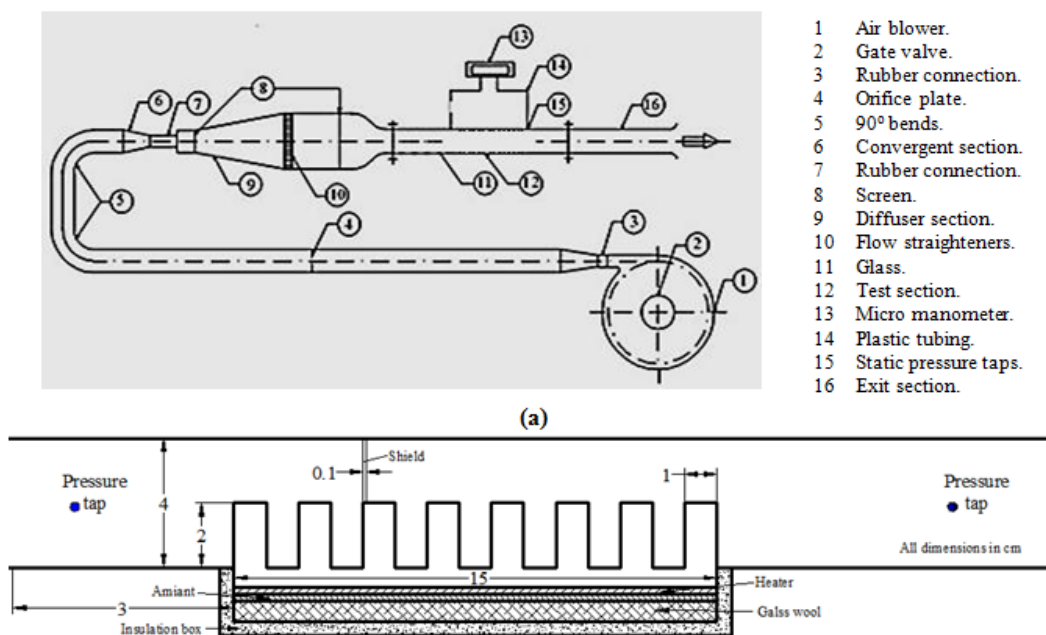
Figure 1. Schematic diagram of (a) test rig and instrumentation (b) test section
