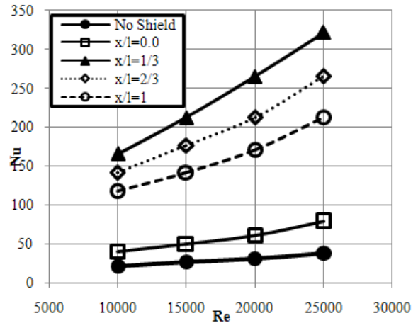
Figure 8. Nusselt numbers versus Reynolds numbers at different shield positions
