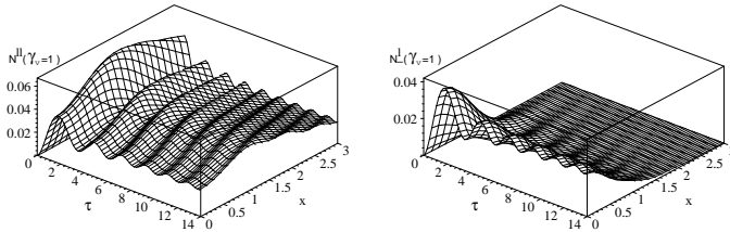
Figure 4: Dependence of longitudinal N^{\parallel} and transverse N^{\perp} components of the distribution function of vector bosons on time \tau = 2h_i\eta and momentum ( x = q/m_i ). Their momentum distributions in units of the primordial mass x = q/M_I show the large contribution of longitudinal bosons. Values of the initial data M_I = H_I follow from the uncertainty principle and give the temperature of relativistic bosons T \sim H_I = (M_0^2 H_0)^{1/3} = 2.7K [63]
