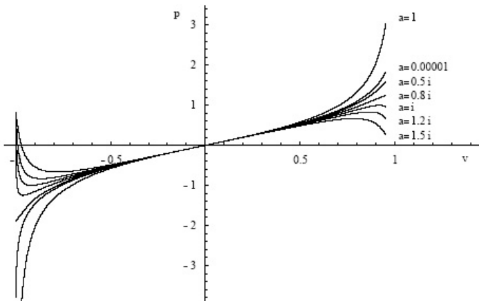
Figure 2: p(1, v) plots for imaginary parameter a = 0.5i, 0.8i, i, 1.2i, 1.5i compared with a = 1 and a = 0.00001 (Plot range is not symmetric).
